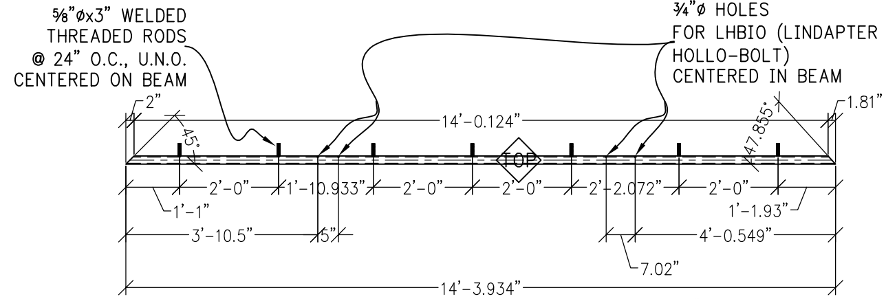
PLAN VIEW
