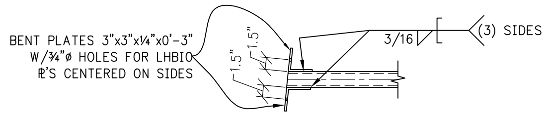
SECTION A
