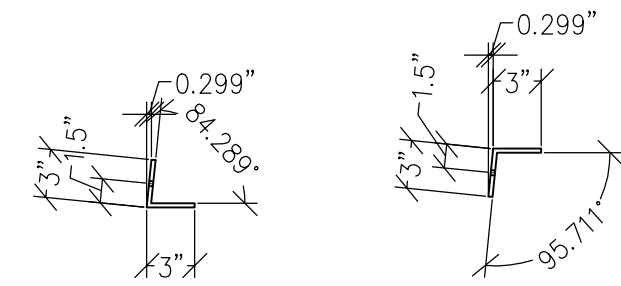
SECTION A
