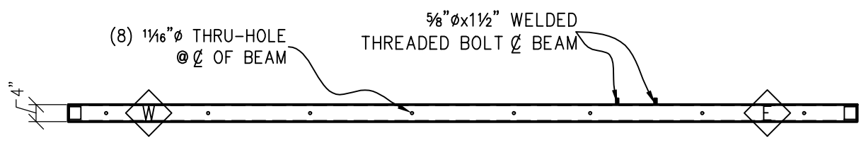
PLAN VIEW
