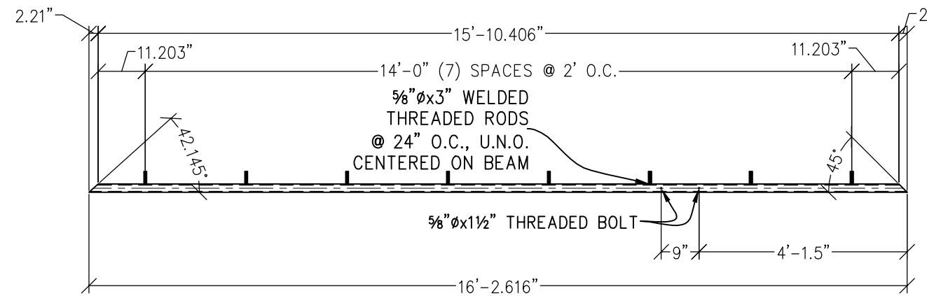
PLAN VIEW
