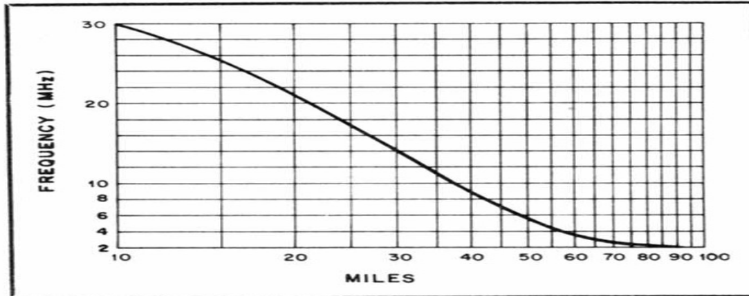
Fig. 1 — Typical high-frequency range, in miles, for ground waves compared to frequency. \text{km} = \text{mi} \times 1.609 .
