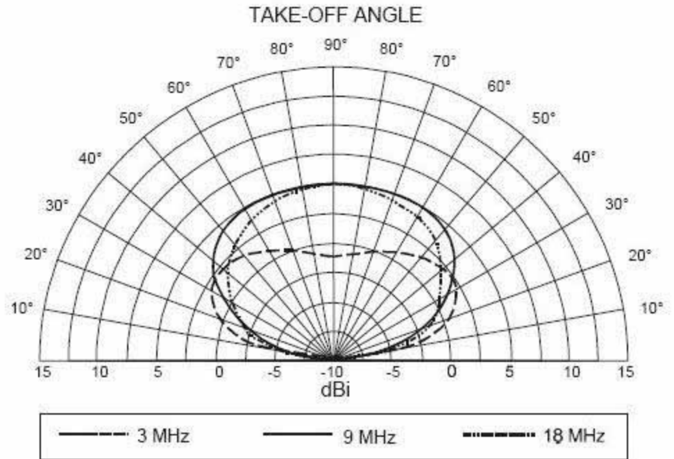
AS-2259 Vertical Radiation Pattern
