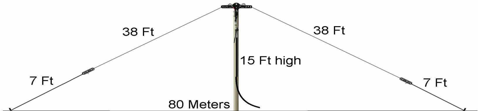
Side Views
