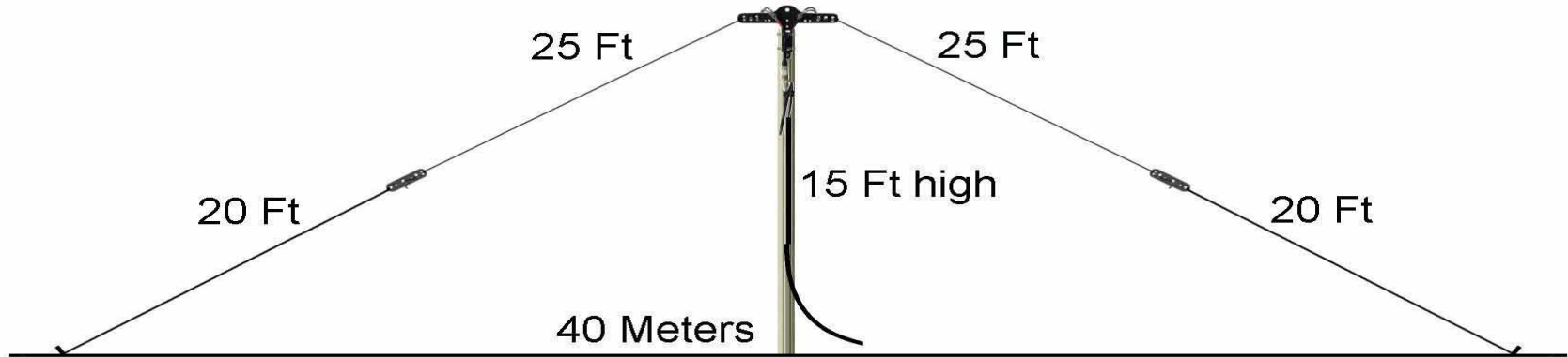
Side Views
