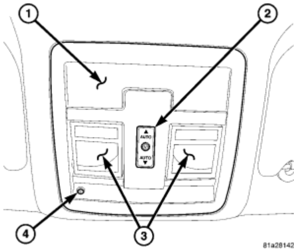
Fig. 1: Identifying Overhead Console, Sunroof Switch, Courtesy Lamps & Infrared Temperature Sensor Courtesy of CHRYSLER LLC
