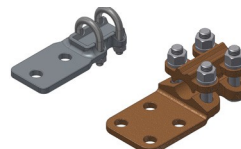
Two or four hole NEMA pads for primary connection
